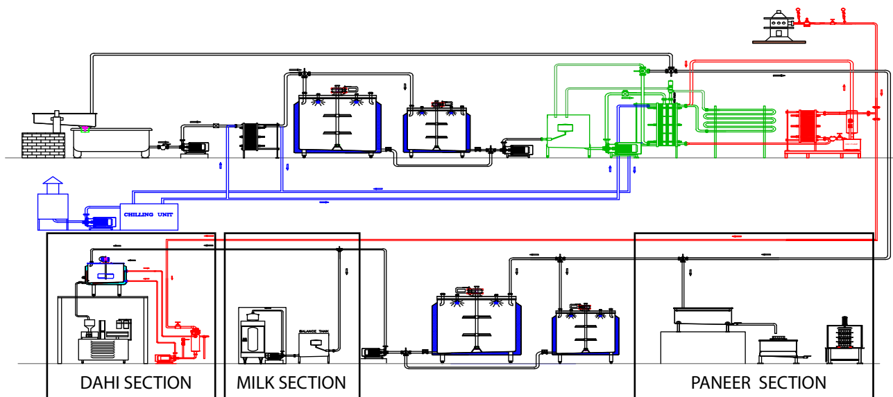
MILK , DAHI & PANEER PLANT LAYOUT
